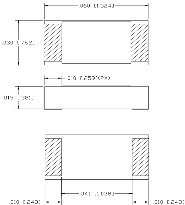
Dimensions in inches [mm] Tolerance ± .005 [.127] unless otherwise stated
